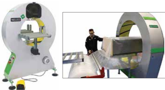
ND - SH - Neleo Orbital Stretch Wrapping Machine - Power Pre-Stretch Fully Automatic / Semi Automatic Options Bubble Wrap / Corrugated Sheet Applicator Optional
