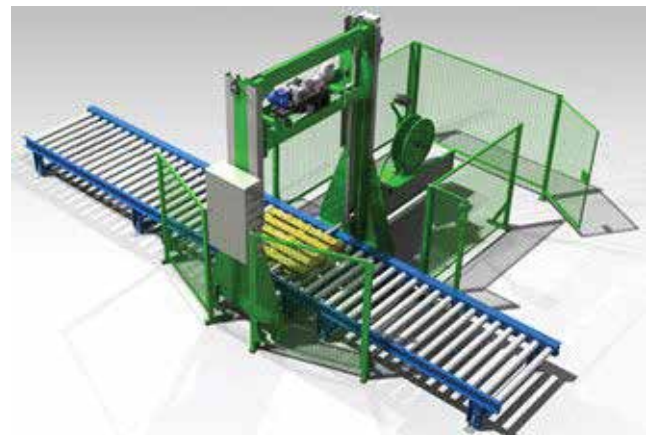
ND - ST - APA014 Automatic Pallet Strapping Machine - Online Manual Intervention Not Required Horizontal / Vertical Strapping Options Available
